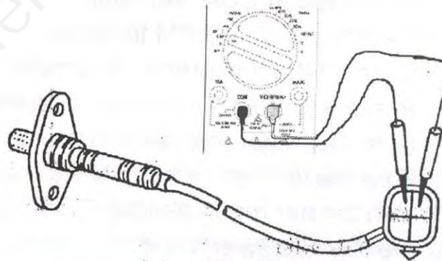
Resistance for testing oxygen sensor heater
